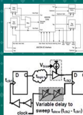
Circuit
